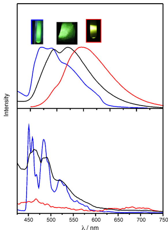
Fig. 11. Emission spectra of fac -[Re(CO) 3 (phen)( cis -bpe)] + (a) and 1,10 phenanthroline (b) in PMMA (black line) or fluid solution (red line) at 298 K, and in EPA (blue line) at 77 K ( inset : emission of the complex according to the environment).
